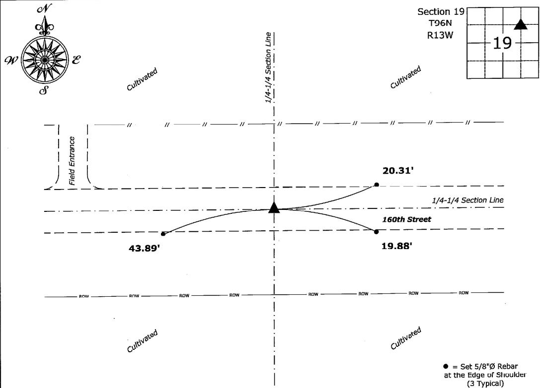
Southwest Corner of the NE 1/4 - NE 1/4 of Section 19-96-13 Found T-Bar
